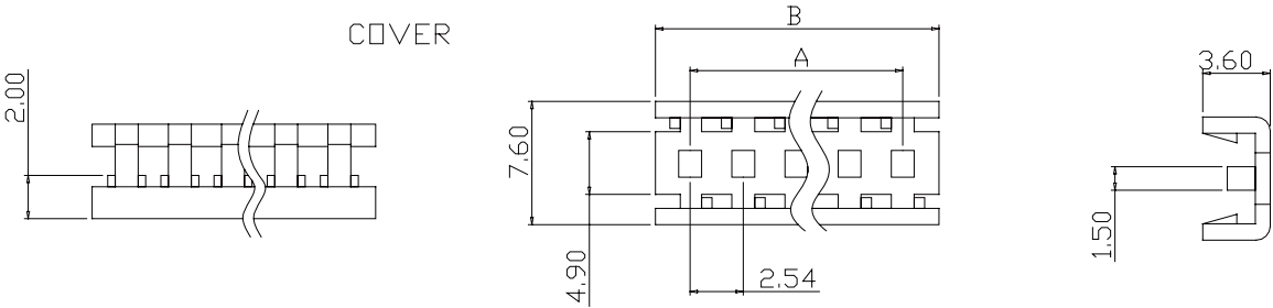
PartNo.:2540IDC-C-L
